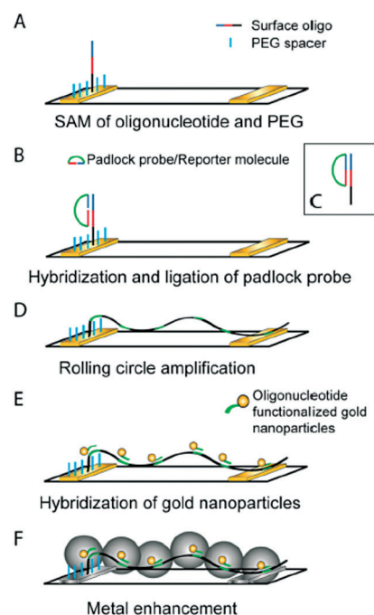
Figure 4. Formation of metalized wires from stretched rolling circle amplification (RCA) products to generate an electrical signal. Reprinted from Ref. [18] with permission. Copyright 2014 American Chemical Society.
