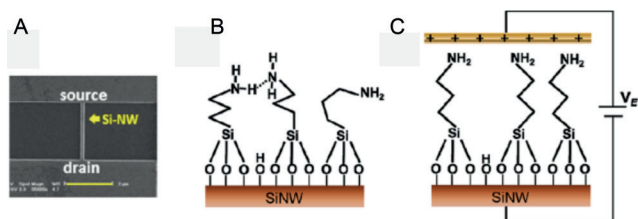
Figure 3. Alignment of aminopropyltriethoxysilane (APTES) on Si NW FETs by an electric field. A) SEM image of a Si NW FET. B,C) Schematic illustrations of the possible APTES molecular structures before and after the alignment process. Reprinted from Ref. [16] with permission. Copyright 2013 American Chemical Society.
