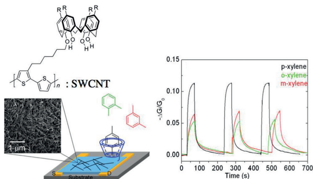
Figure 11. Schematic view of the SWCNT/polymer sensor that selectively adsorbs p -xylene. Reprinted from Ref. [203].
